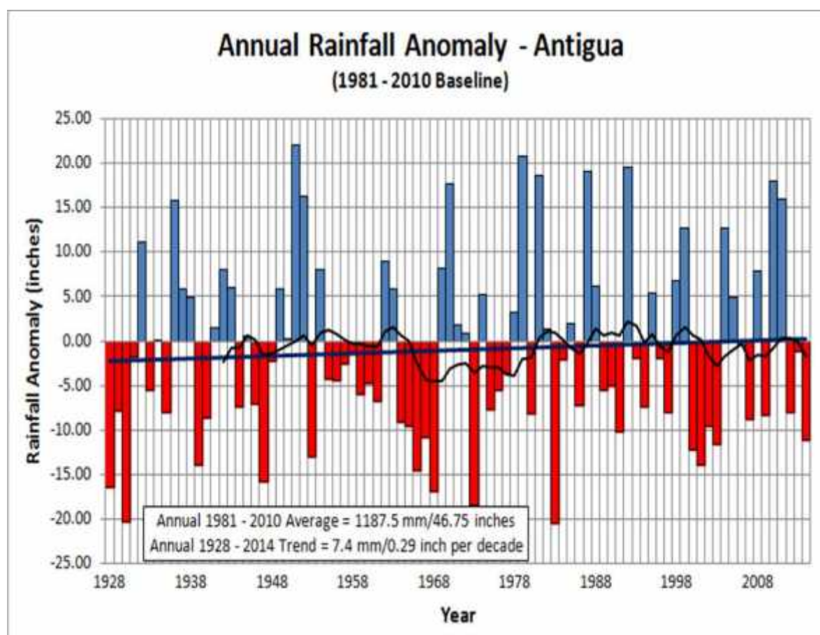
Figure 3 Annual Rainfall Anomaly for Antigua
